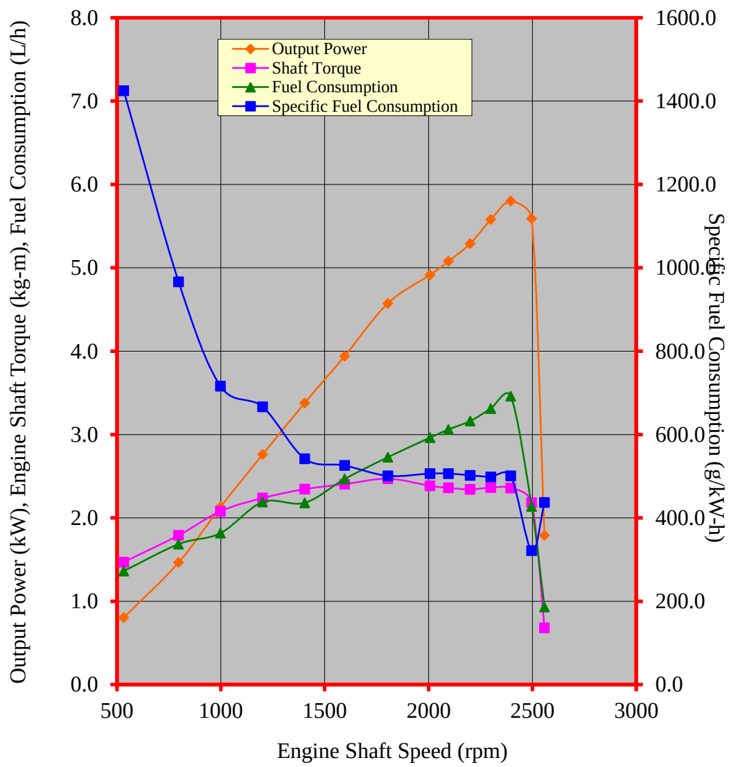
Figure 3. Performance characteristic curves of the KUVICO KV80 diesel engine
