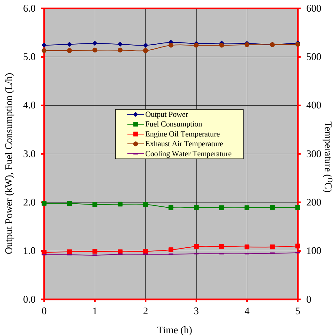
Figure 4. Performance characteristic curves during the continuous running test of the KUVICO KV80 diesel engine
